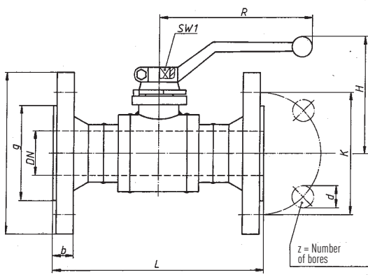
DN 32-100 ▲
